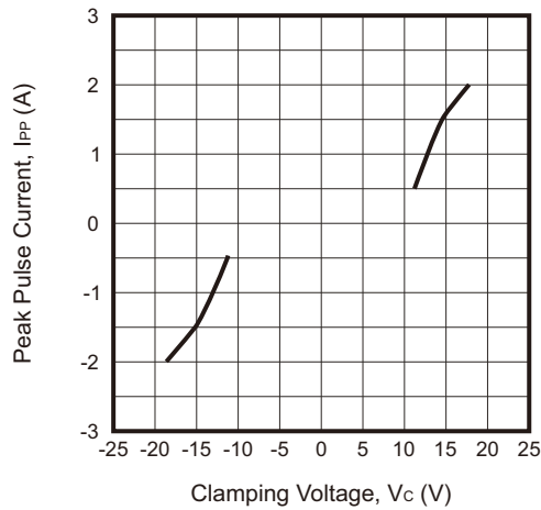
Fig.1 - Clamping Voltage Curve
