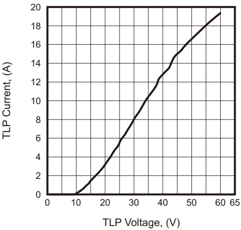
Fig.2 - TLP-Positive Pulse
